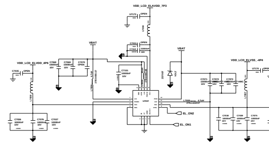
OCTA DCDC
