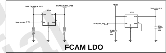
FRONT_24M CAMERA(30PIN)_IMX576_18.06.14
