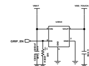
Grip Sensor
