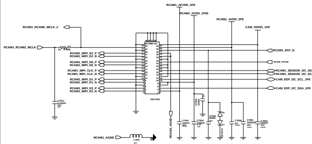
RCAM1_24M CAMERA(34PIN)_IMX576
