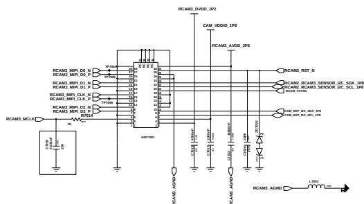
RCAM3_SUPER WIDE_8M CAMERA(30pin)_S5K4HA
