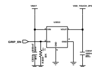
Grip Sensor
