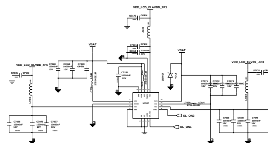
OCTA DCDC
